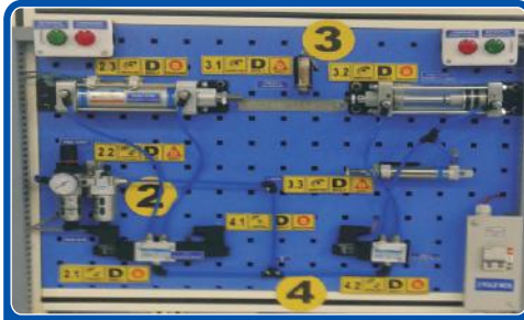
PNEUMATIC TRAINING KIT
